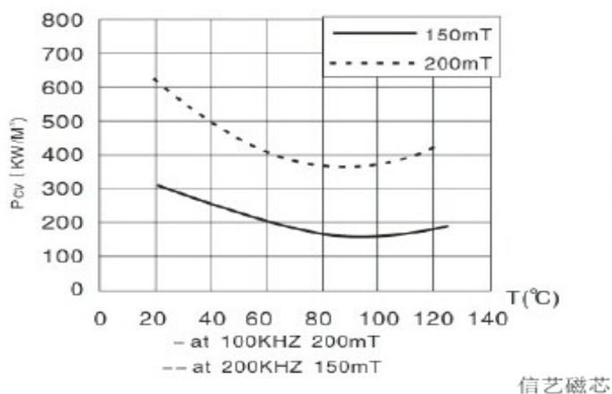
功率损耗的温度特性曲线 Power Loss vs temperature
